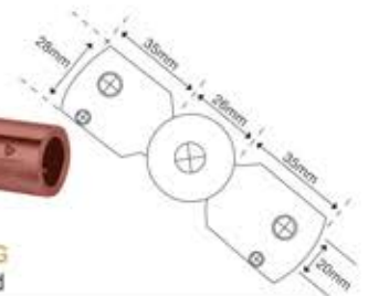
DFKH-3 RG Rod to Rod
