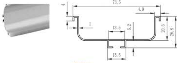
DFWP-5 C-Profile Gola Colour : Anodized, CP Finish, Brush CP, SS Brush Rose Gold, Black Matt, Gold Matt, Gold Glossy
