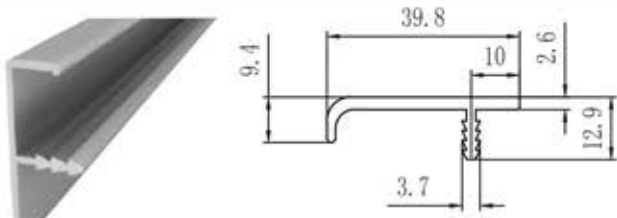
DFWP-7 MY-A673S F-Wooden Handle Profile Colour : Anodized, CP Finish, Brush CP, SS Brush Rose Gold, Black Matt, Gold Matt, Gold Glossy
