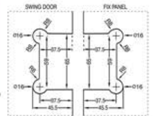
DFSH-44 RG Glass to Glass 90° Hinge
