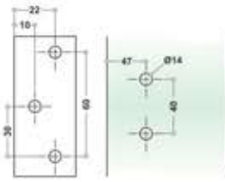
DFCFS-2 Glass to Wall Hinge
