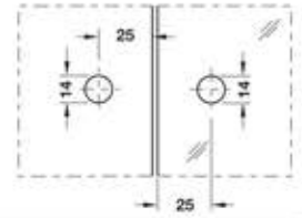
DFGC-22 RG Glass to Glass 135°
