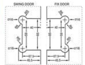
DFSH-33 RG Glass to Glass 135° Hinge
