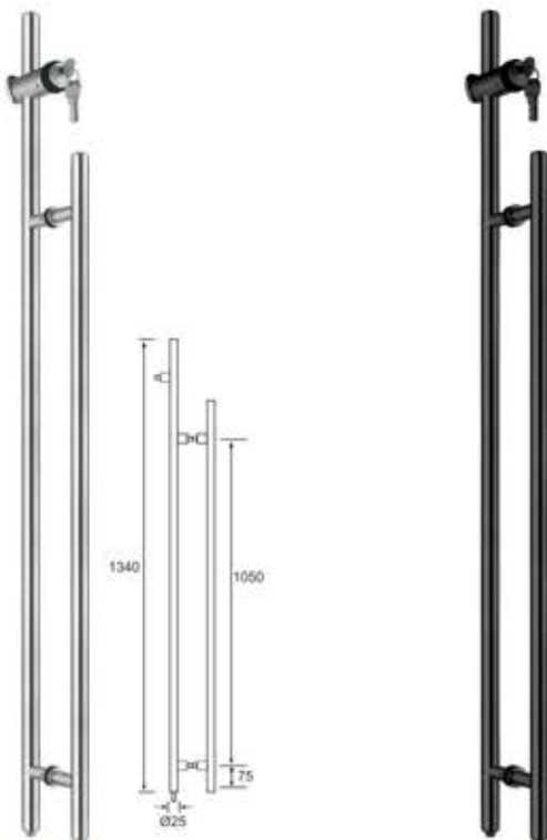
DFDHL-66 Size : 25x1340mm DFDHL-55 BM Size : 25x1340mm
