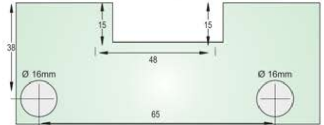
CUTOUT DETAILS OF SSL-44-R8
