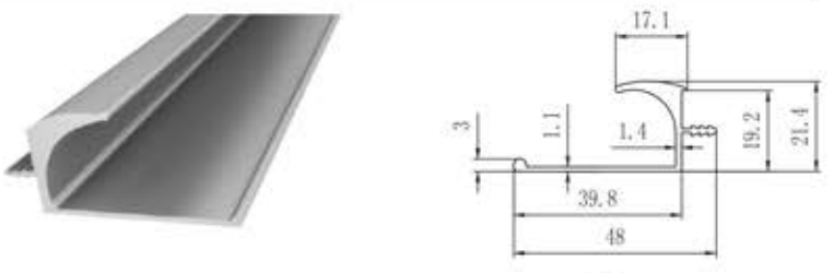
DFWP-4 K1347 J-Wooden Handle Profile Colour : Anodized, CP Finish, Brush CP, SS Brush Rose Gold, Black Matt, Gold Matt, Gold Glossy
