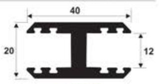
DGEF-4 For Glass Door Partition
