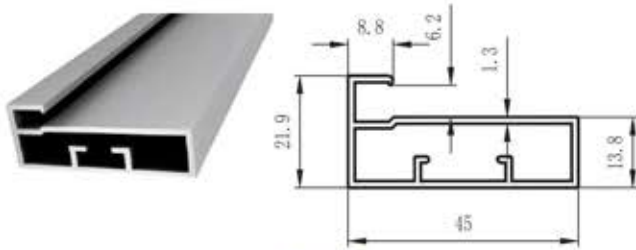
DFWP-1 Frame Profile 45mm Colour : Anodized, CP Finish, Brush CP, SS Brush Rose Gold, Black Matt, Gold Matt, Gold Glossy
