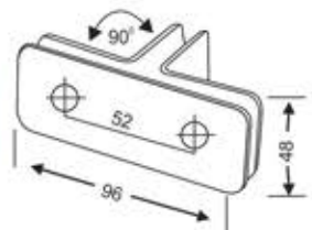
DFGC-66 RG T-Connector Glass to Glass 90°
