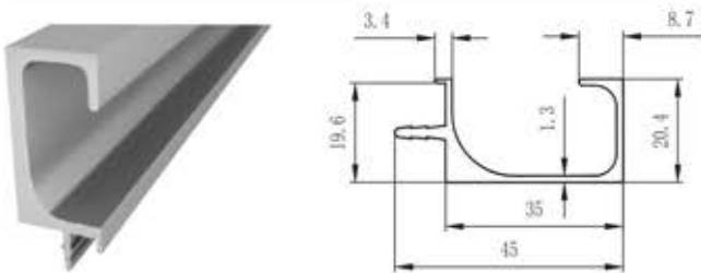
DFWP-3 G-Wooden Handle Profile Colour : Anodized, CP Finish, Brush CP, SS Brush Rose Gold, Black Matt, Gold Matt, Gold Glossy
