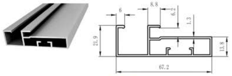
DFWP-2 Handle Profile for 45mm Frame Colour : Anodized, CP Finish, Brush CP, SS Brush Rose Gold, Black Matt, Gold Matt, Gold Glossy
