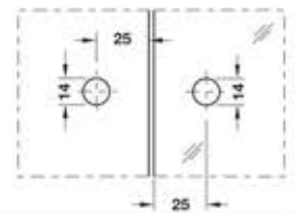
DFGC-55 RG Glass to Glass 180°
