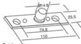
DFPL-2B Centre Lock Strike Box
